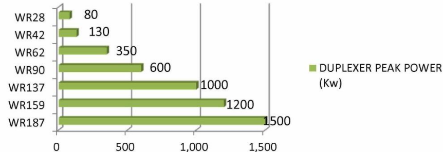
DUPLEXER PEAK POWER (Kw) @ 1 ATM.
